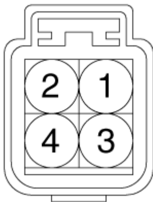
Harness Connector
